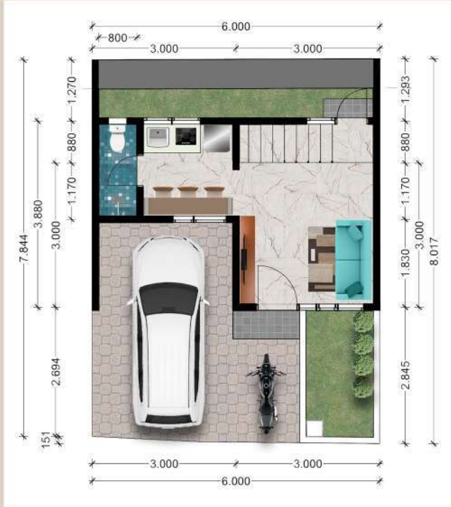
DENAH LANTAI 1
