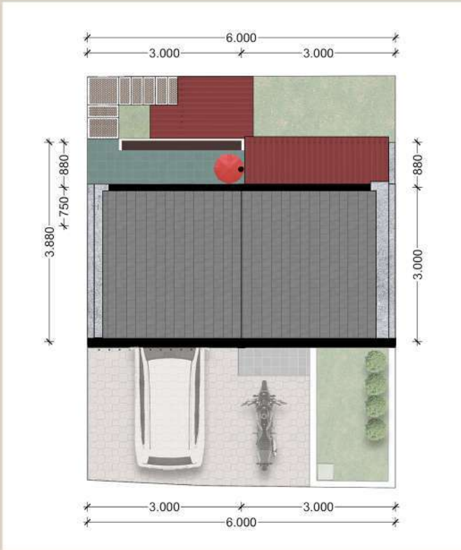
DENAH ROOFTOP
